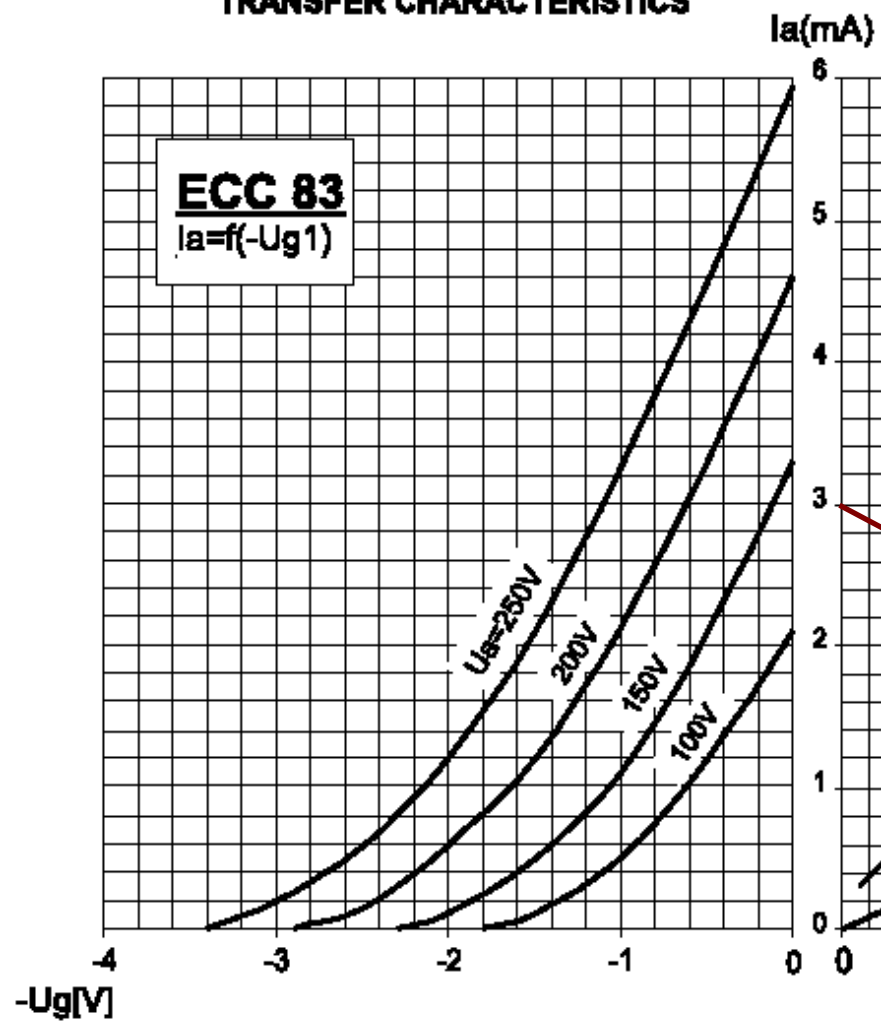
TRANSFER CHARACTERISTICS
