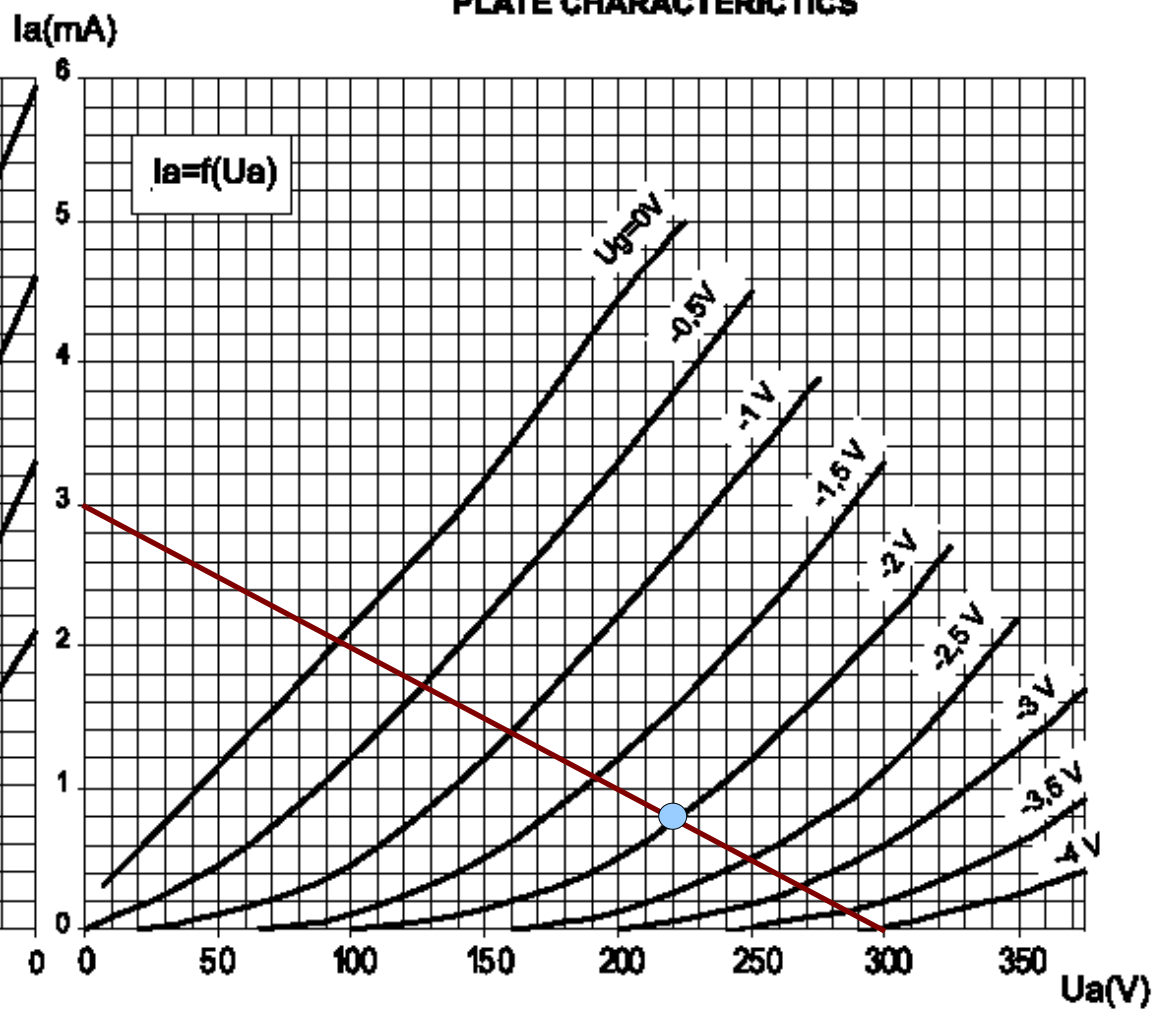
PLATE CHARACTERISTICS
