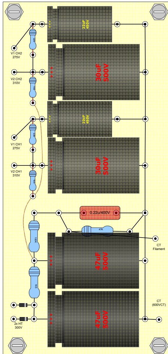
HV PSU incl. Heater Elevation
