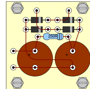
Unregulated 5VDC PSU
