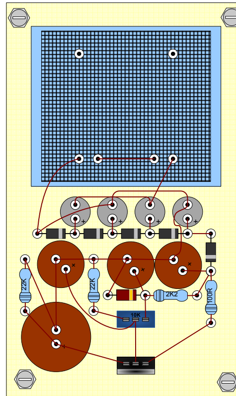
Adjustable Phantom Power Supply
