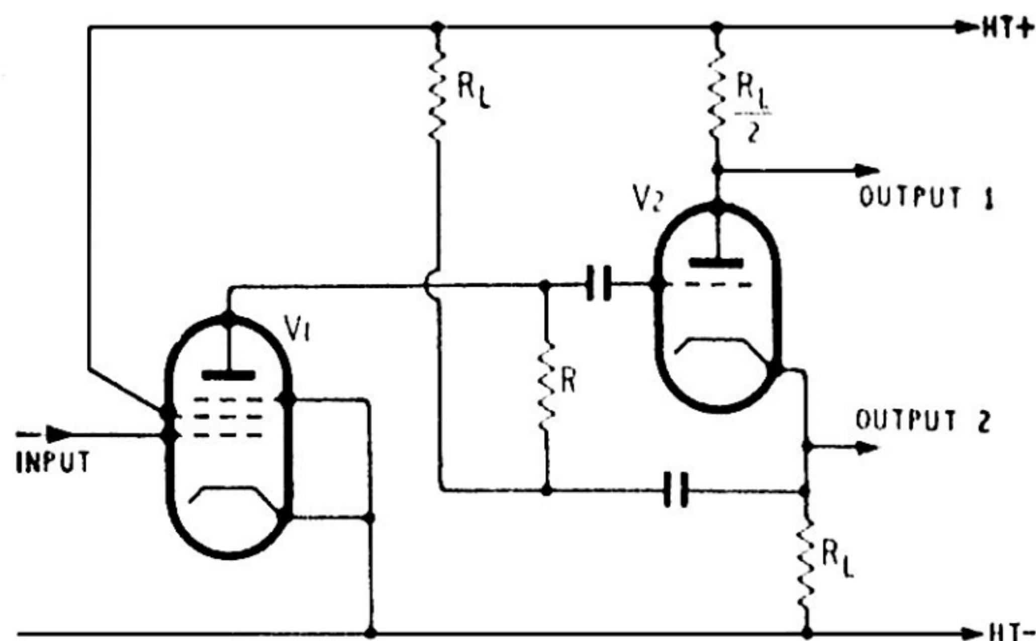
Fig. 4. Basic circuit of Jeffery's high-gain phase-splitter.
