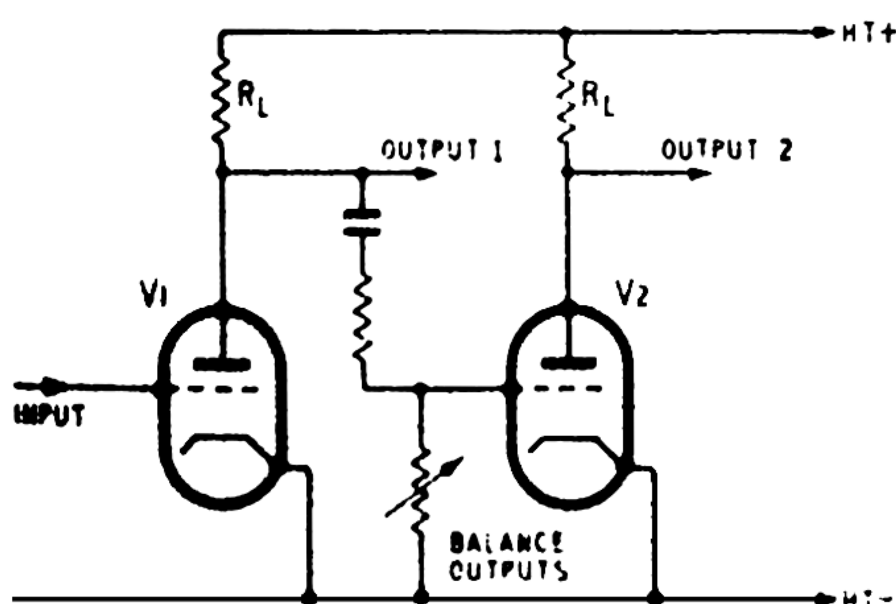
Fig. 1. Basic circuit of paraphase phase-splitter.
