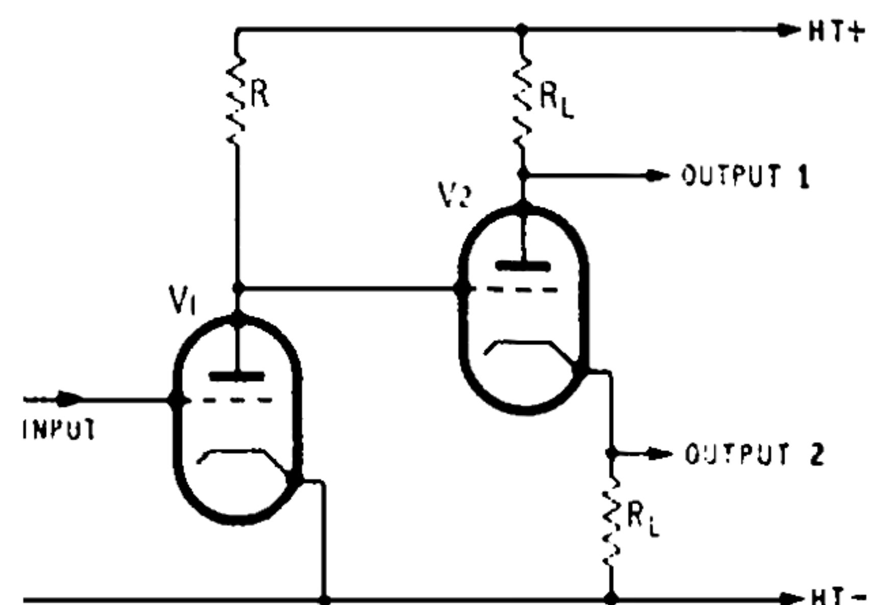
Fig. 3. Basic circuit of direct-coupled concertina phase-splitter.
