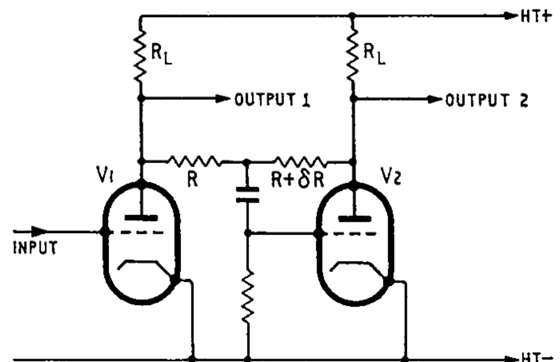
Fig. 2. Basic circuit of "floating" paraphase phase-splitter.
