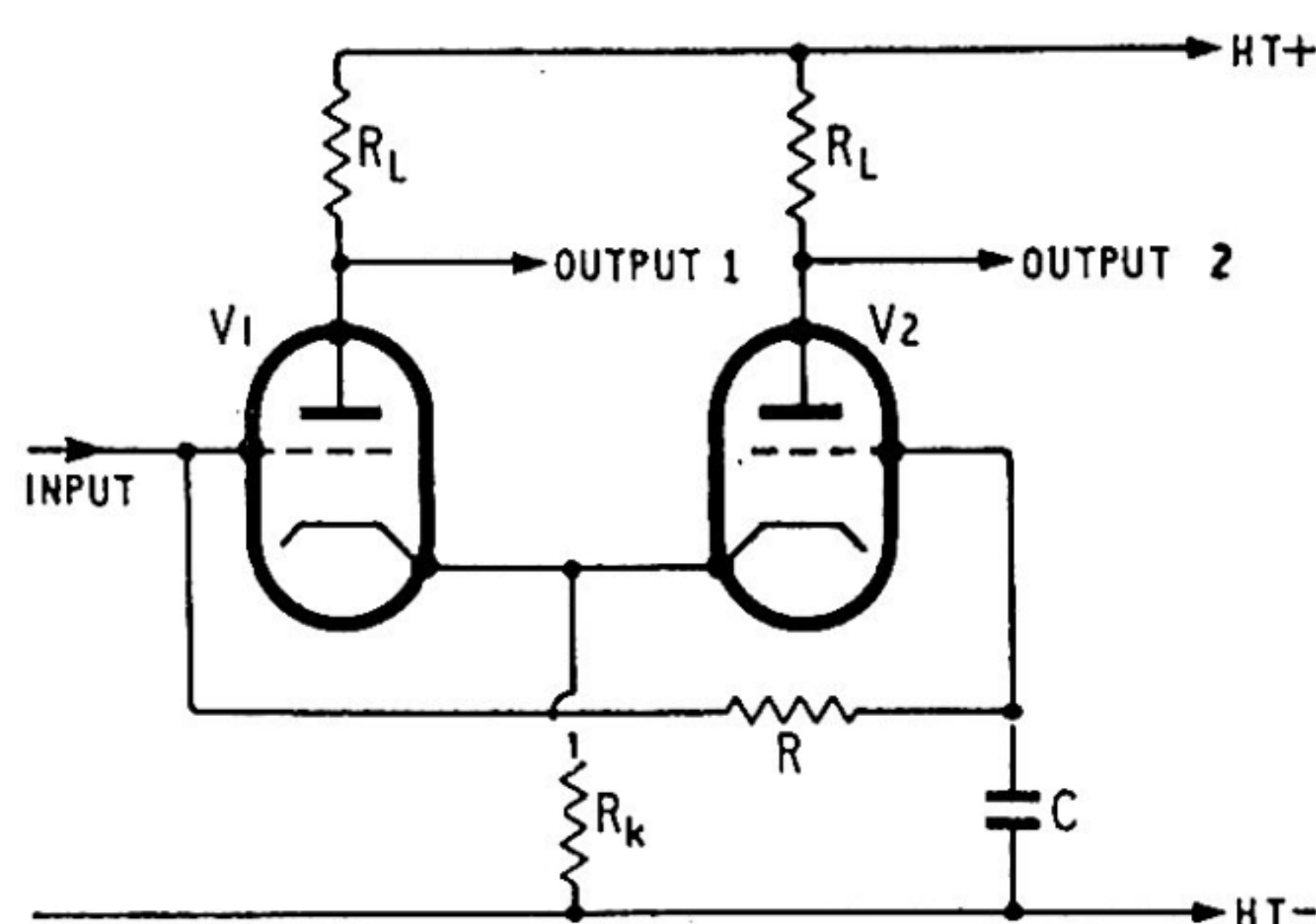
Fig. 5. Basic circuit of long-tailed-pair phase-splitter.
