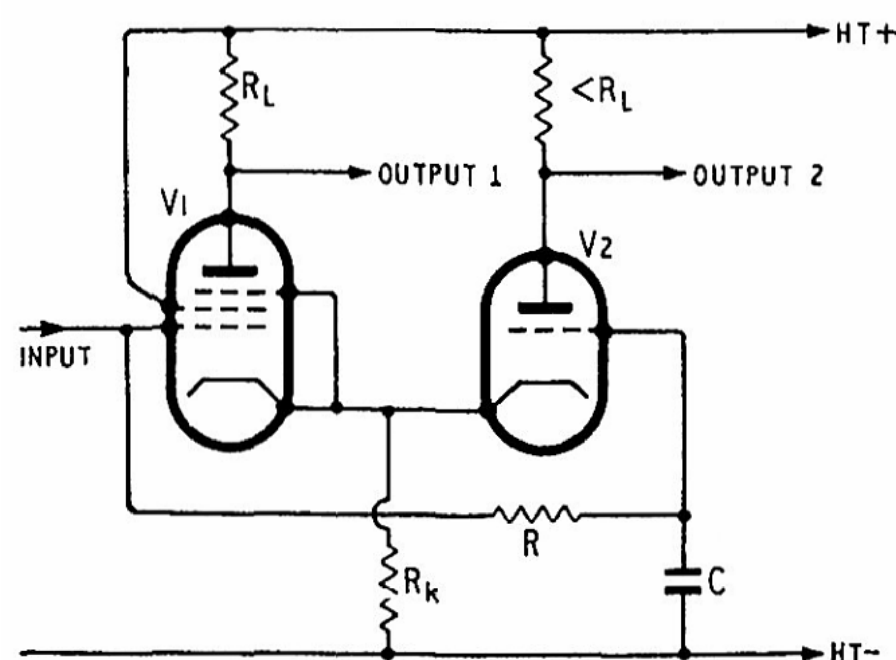
Fig. 6. Basic circuit of modified long-tailed-pair phase-splitter.
