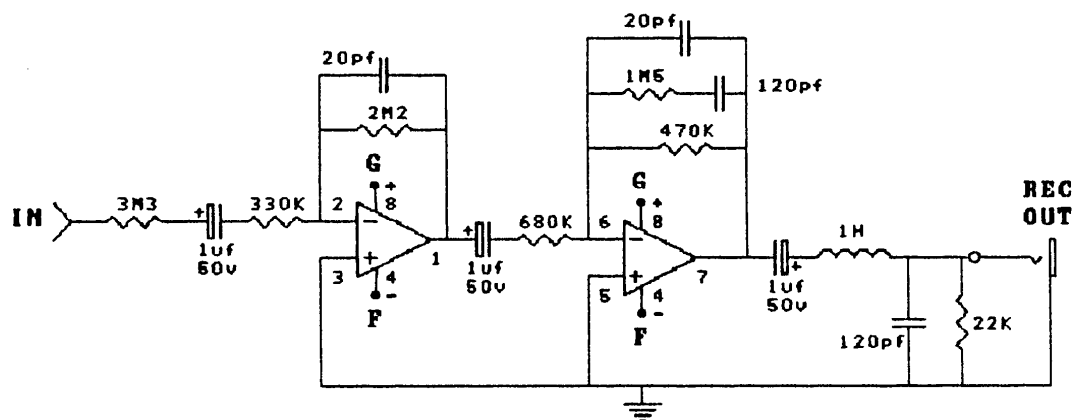
RECORD OUT CIRCUIT - TL072
