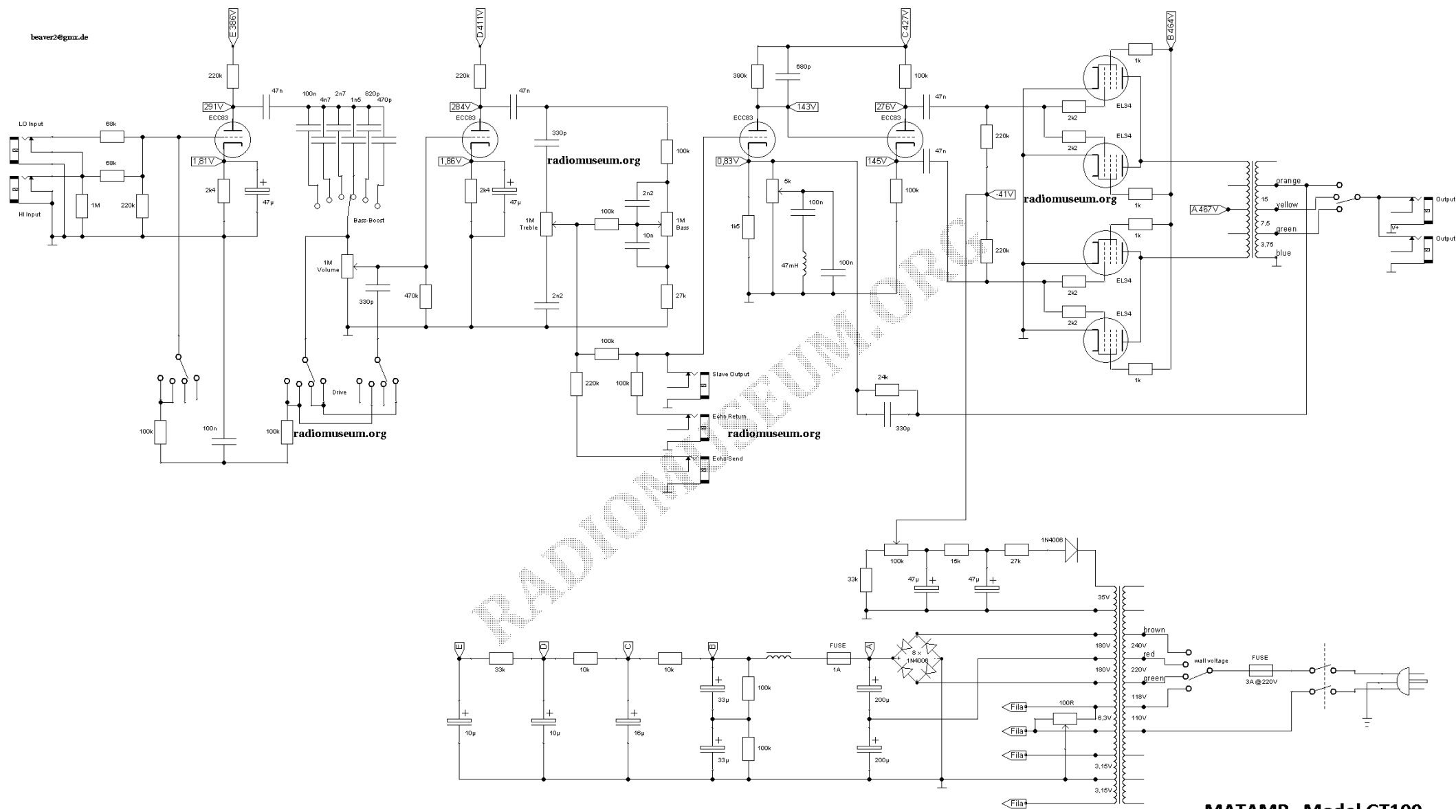
MATAMP Model GT100
