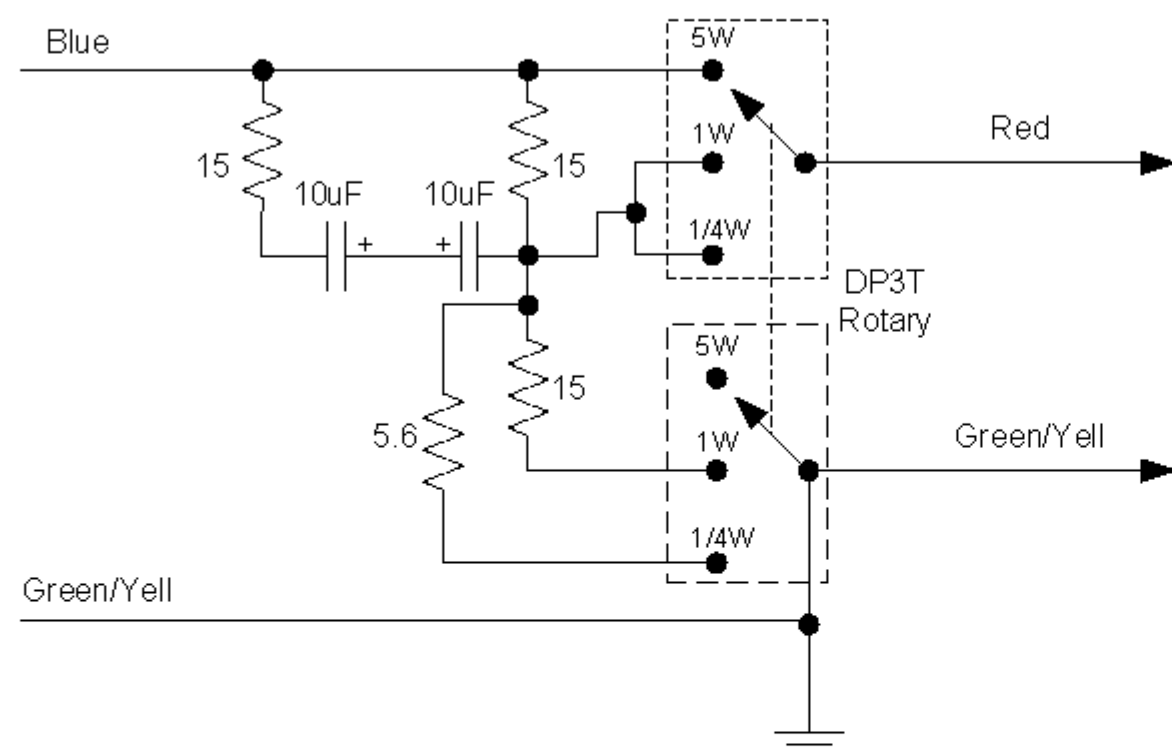
Attenuator Network
